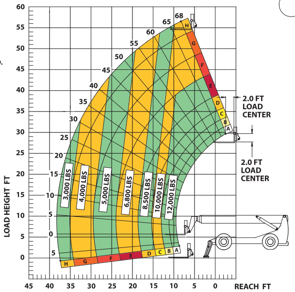
XR1255 LOAD CHART OUTRIGGERS DOWN - STANDARD CARRIAGE
