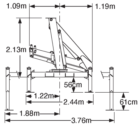
STOWED POSITION AND STABILIZER DIMENSIONS (1 HYD EXTENSION)
