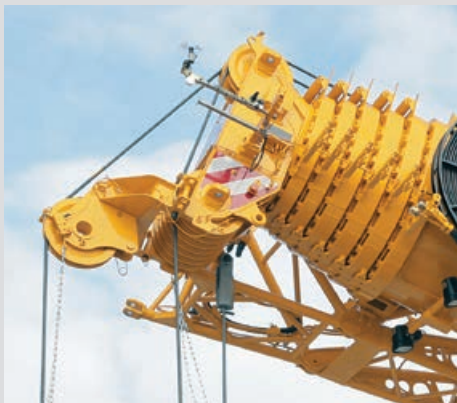
Rooster sheave, foldable sidewise
