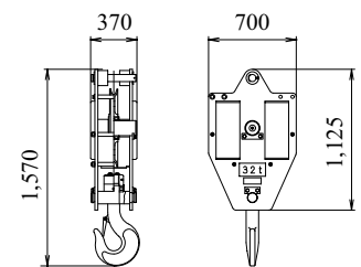
32 t Hook Weight: 400 kg
