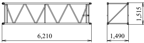
6.1 m Boom Insert Weight: 522 kg
