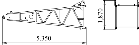
Boom Base Weight: 1,130 kg
