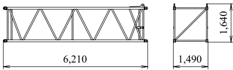
6.1 m Boom Insert with Lug Weight: 545 kg
