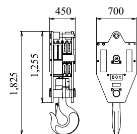
80 t Hook Weight: 650 kg
