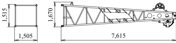
Boom Tip Weight: 1,390 kg
