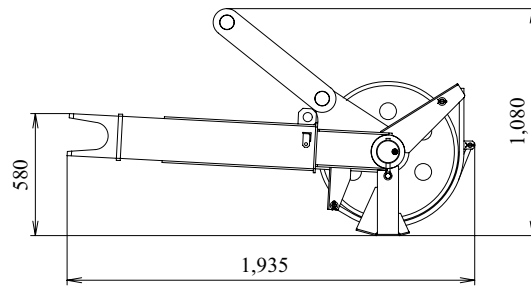
Auxiliary Sheave Weight: 330 kg
