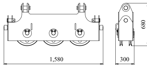
Upper Spreader Weight: 280 kg
