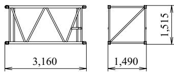
3.0 m Boom Insert Weight: 310 kg
