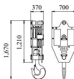
50 t Hook Weight: 500 kg
