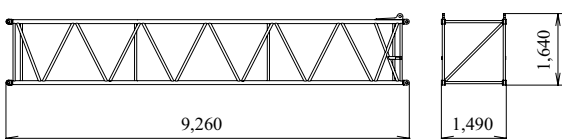
9.1 m Boom Insert with Lug Weight: 765 kg
