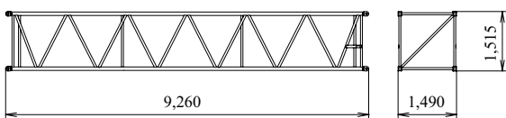
9.1 m Boom Insert Weight: 745 kg
