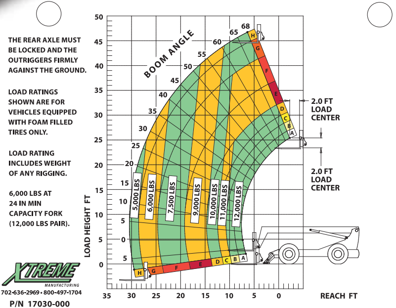
XR1245 LOAD CHART OUTRIGGERS DOWN- STANDARD CARRIAGE
