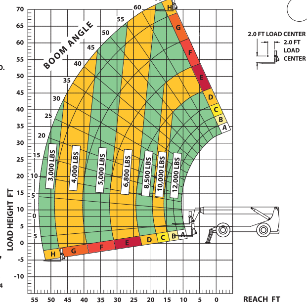
XR1270 LOAD CHART OUTRIGGERS DOWN - STANDARD CARRIAGE
