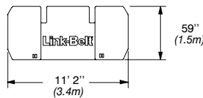
Upper Counterweight "B" – 25,350 lbs. (11 499kg)
