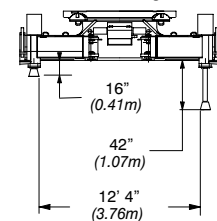
Carbody Jack minimum and maximum heights
