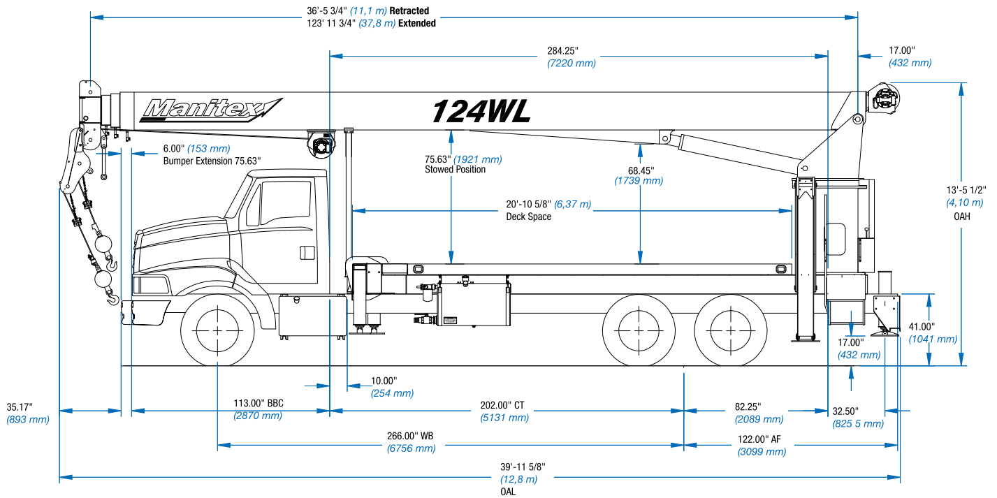
Typical Wireline configuration, does not reflect minimum truck requirement
