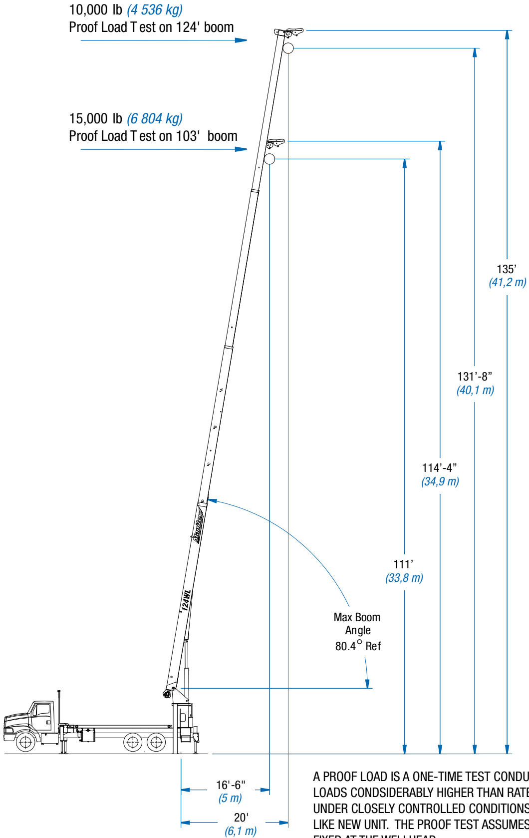
PROOF LOAD TEST DIAGRAM Model 124WL
