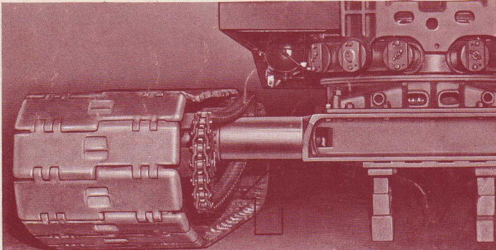
Machined axles allow extending or retracting crawler side frames for minimum width when transporting (machine can be propelled when crawlers are in retracted position).
