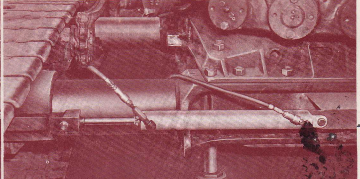
Optional hydraulic counterweight removal device consists of two cylinders which attach to the rear of the cab. This same equipment is used for extension or retraction of the crawler frames.
