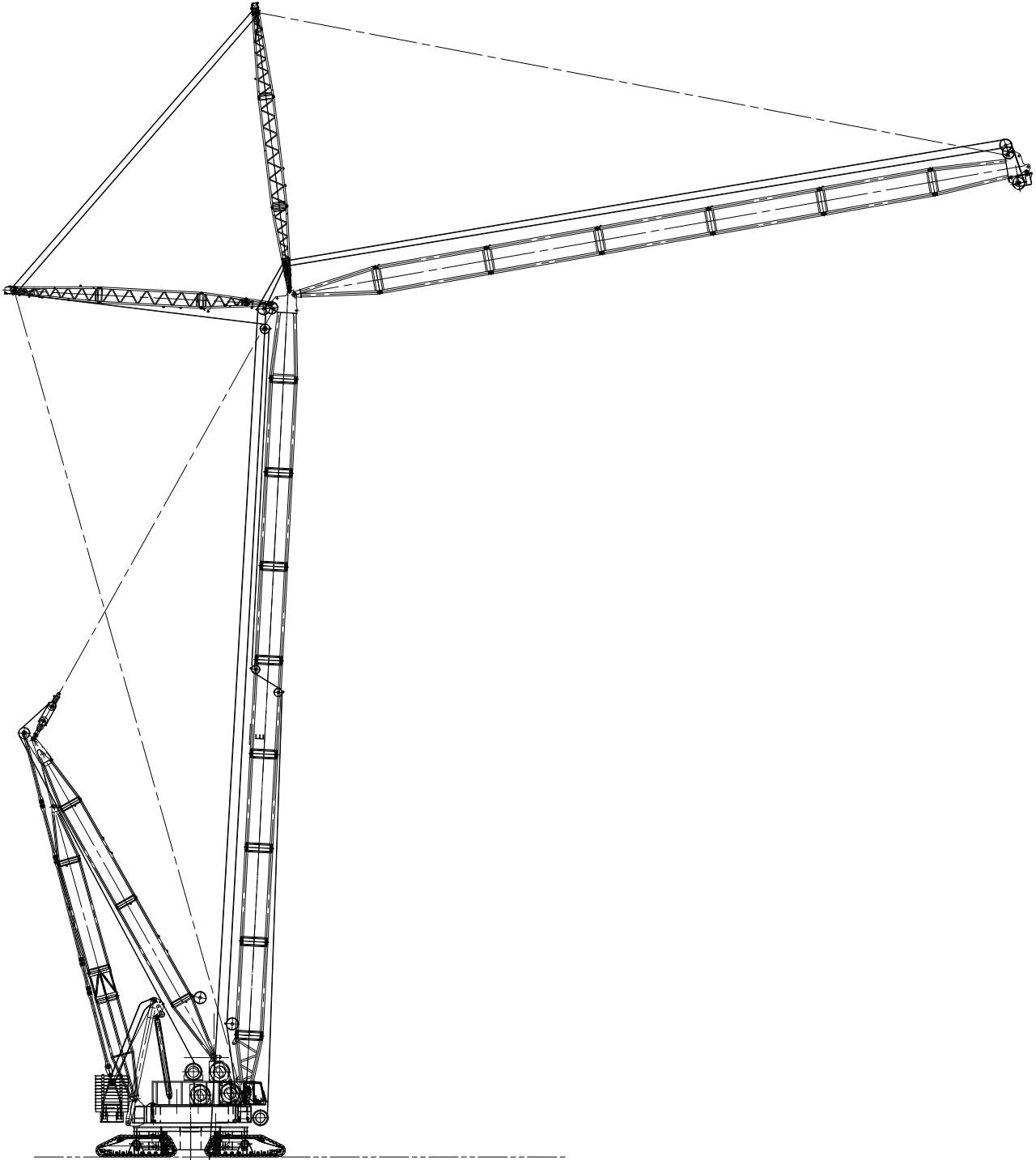
Model 3100 No. 90 Luffing Jib on No. 91 Heavy-Lift Main Boom 95 m + 102 m (646.3 ft)
