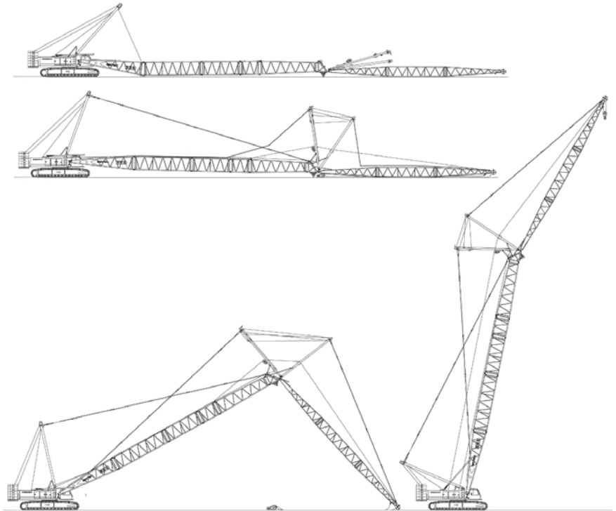
Assembly of boom frame and anchoring rods
