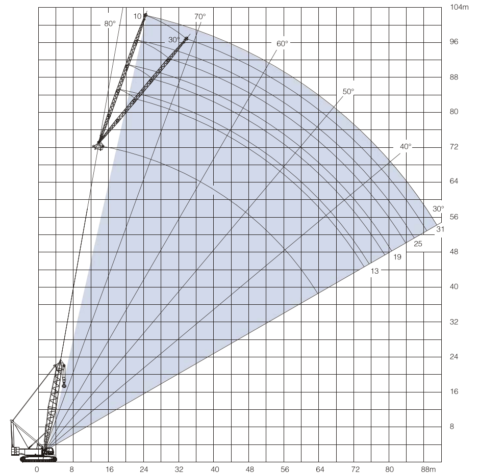
Lifting height on SF boom
